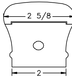
LJ-6210 PROFILE
