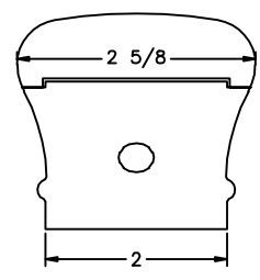
LJ-6210 PROFILE
