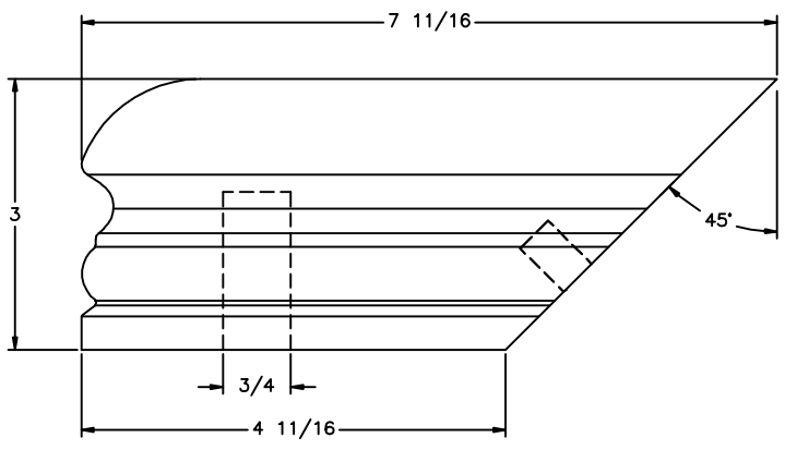
LJ-6519 PROFILE
