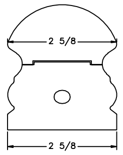
LJ-6519 PROFILE
