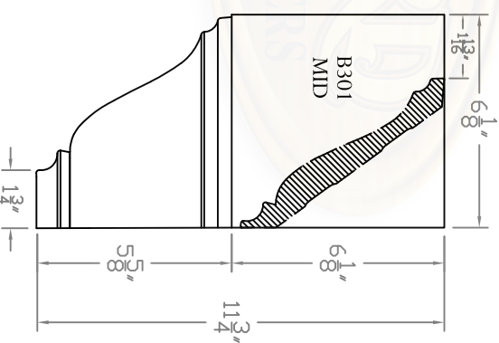
SIDE VIEW MID Scale: 1:4
