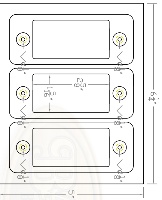
SP1090 (BACK VIEW)
