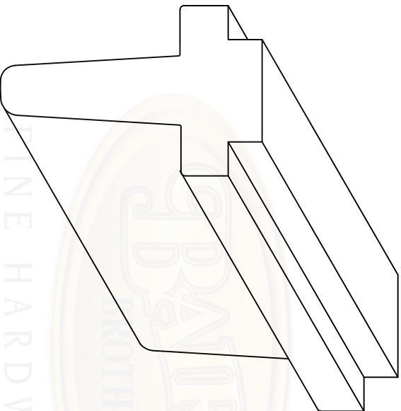
SPL 9654 A 1 3/8 Shaker Style Astragal
