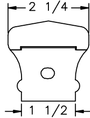
LJ-6601 PROFILE
