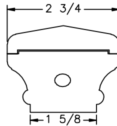
LJ-6701 PROFILE
