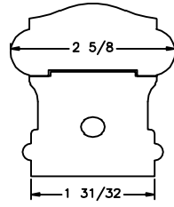
LJ-6900 PROFILE
