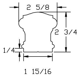
LJ-6900 PROFILE
