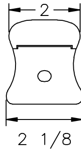
LJ-6010 PROFILE
