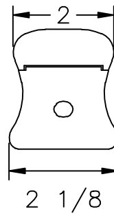
LJ-6A10 PROFILE
