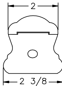
LJ-6B10 PROFILE
