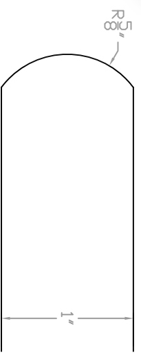
BULLNOSE DETAIL
